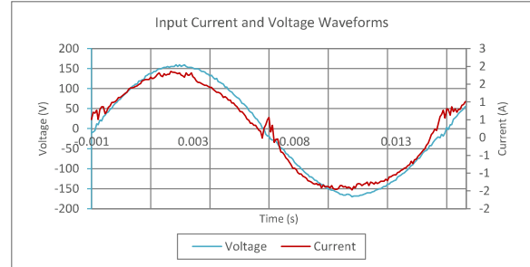
Input AC Current Waveform (ITHD = 6.92%, 50% Load)
